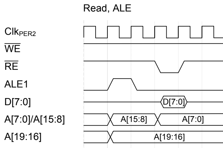
Figure 33-28. Read, ALE
