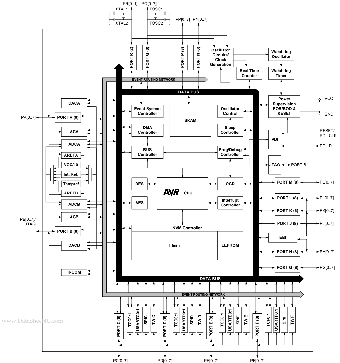
Figure 2-1. XMEGA A Block Diagram
