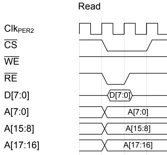
Figure 33-16. Read
