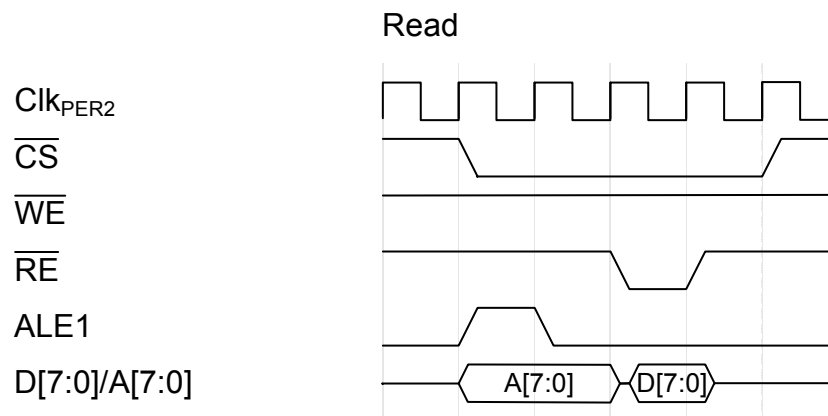
Figure 33-24. Read
