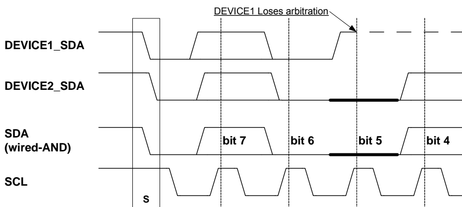
Figure 19-9. TWI Arbitration
