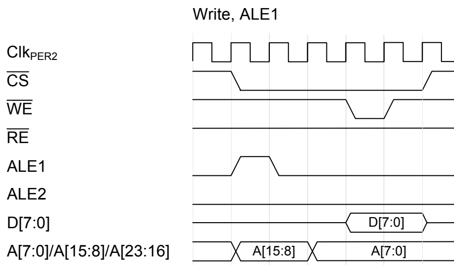
Figure 33-6. Write, ALE1
