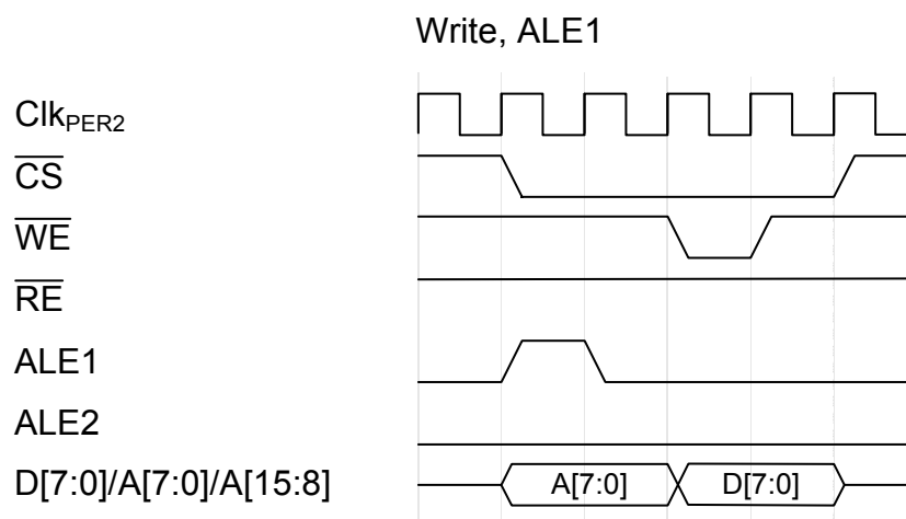
Figure 33-31. Write, ALE1
