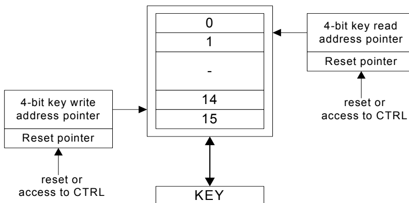
Figure 23-3. The Key memory with pointers and register.
