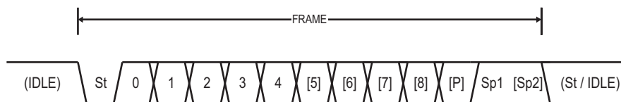
Figure 21-5. Frame Formats
